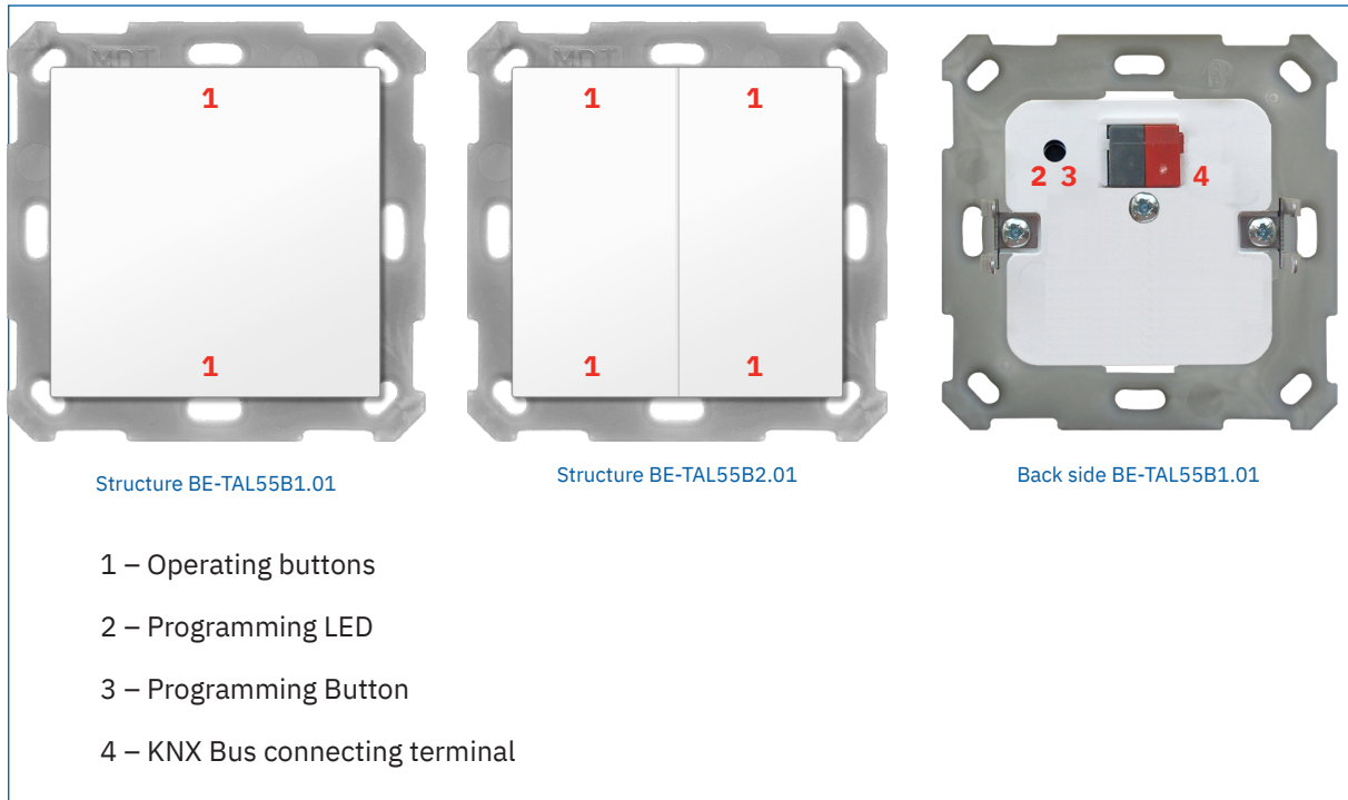
Figure 3: Structure and Handling – Push Button Lite 55 Basic
