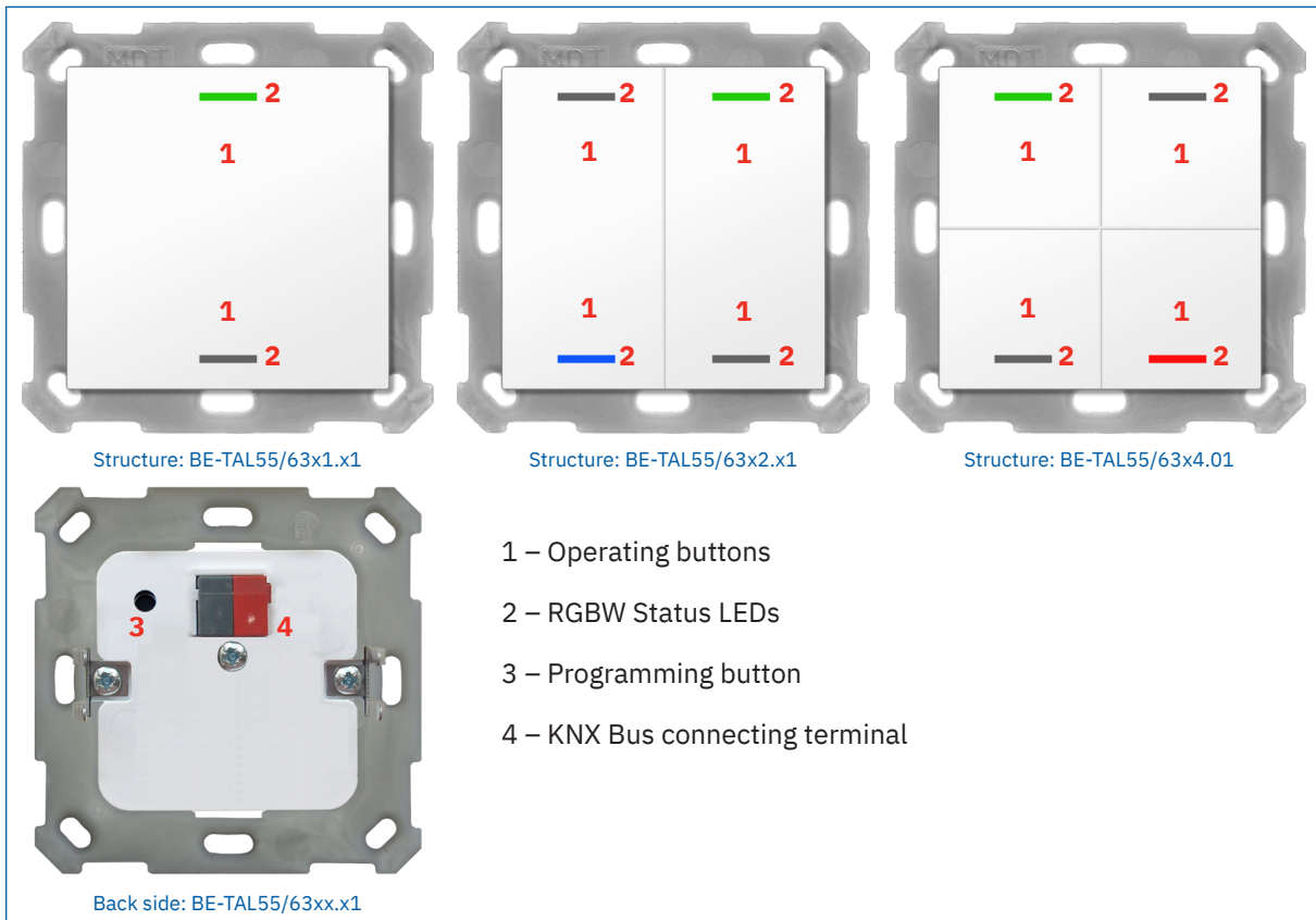
Figure 2: Structure and Handling – Push Button Lite 55/63
