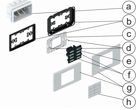
Installation for rectangular flush mounting box
