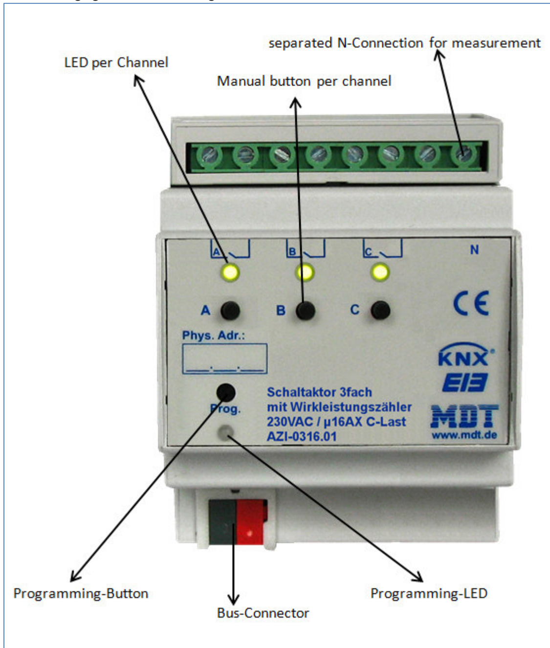
Figure 1: Overview Hardware
