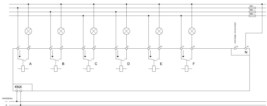
Exemplary circuit diagram AZI-0616.01
