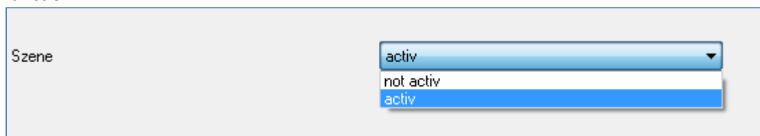
Figure 9: Scene function
