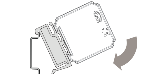
b) Place the support clamping tooth on the top edge of the mounting rail and rotate device and support towards the guide until it completely engages
