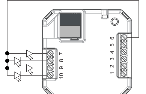
Connection of outputs (low-consumption LEDs)
