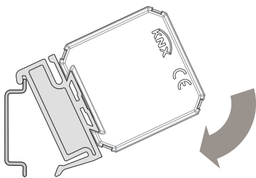
b) Place the support clamping tooth on the top edge of the mounting rail and rotate device and support towards the guide until it completely engages
